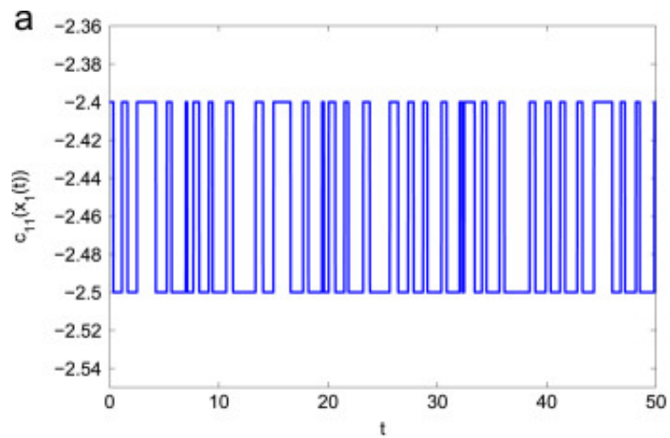
Trajectory of connection weight coefficient c_{11}(x_1(t))
