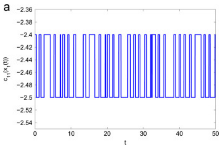
Trajectory of connection weight coefficient c_{11}(x_1(t))
