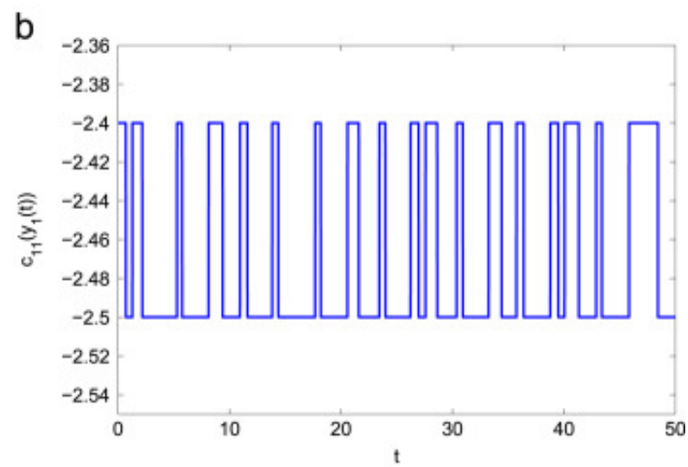
Trajectory of connection weight coefficient c_{11}(y_1(t))
